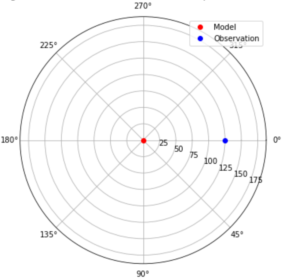
Taylor Diagram - Bushehr Station model (Precipitation-CNRM-SSP.370)
