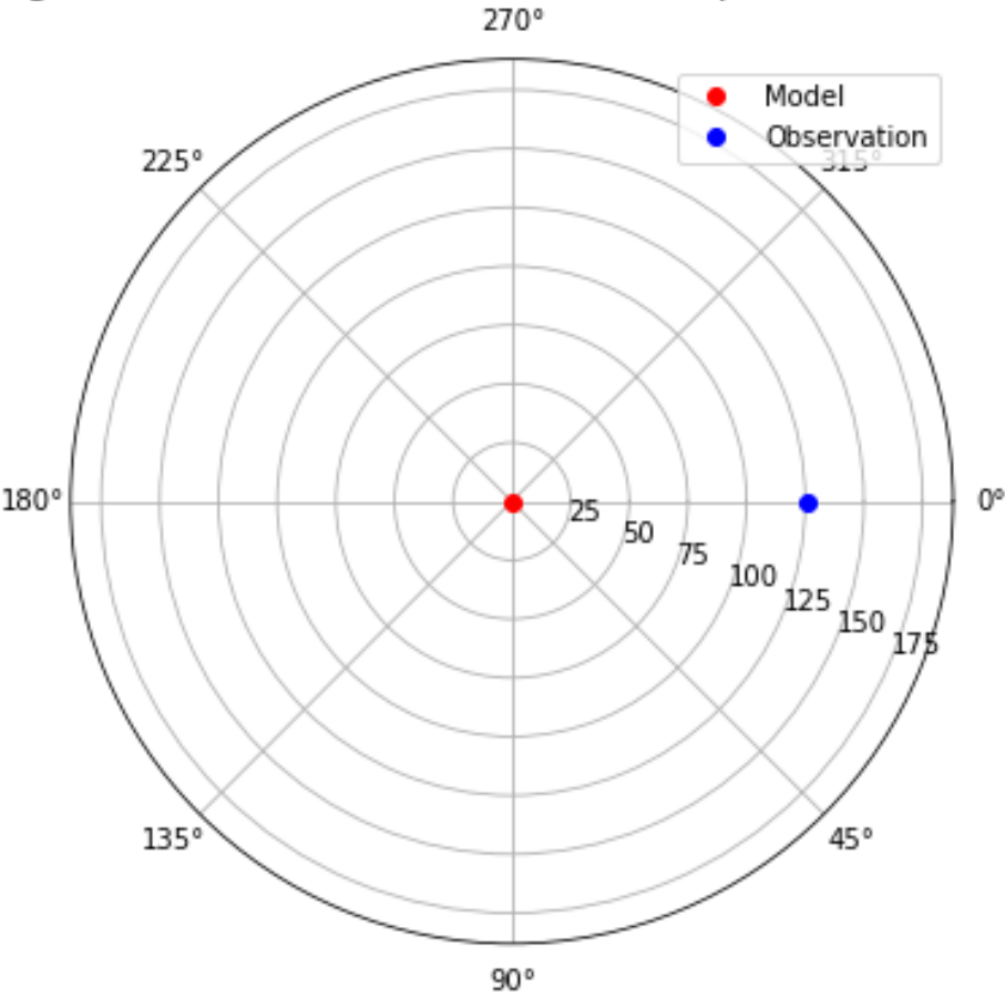
Taylor Diagram - Bushehr Station model (Precipitation-CESM2-SSP.585)
