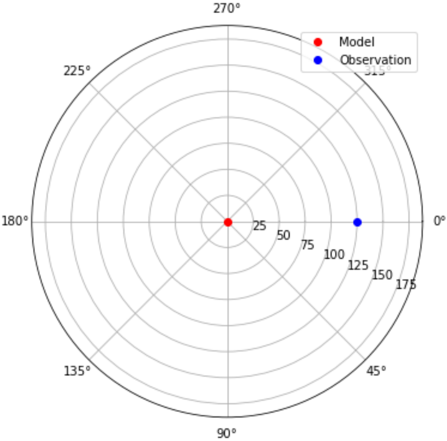
Taylor Diagram - Bushehr Station model (Precipitation-CNRM-SSP.585)
