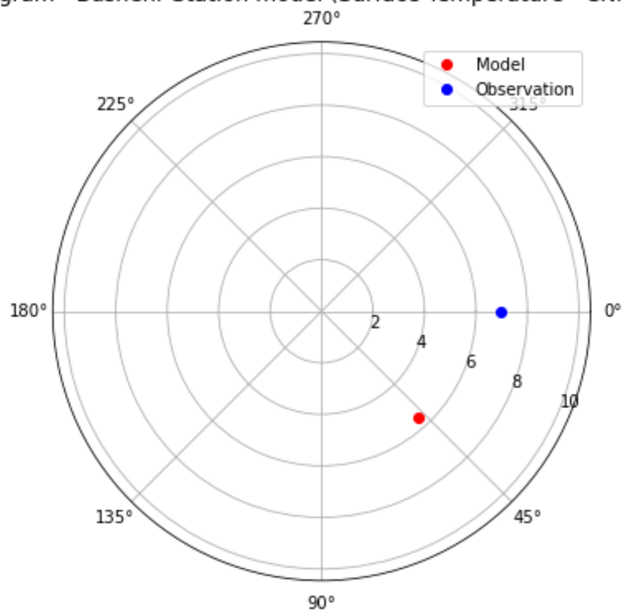
Taylor Diagram - Bushehr Station model (Surface Temperature - CNRM-SSP.370)
