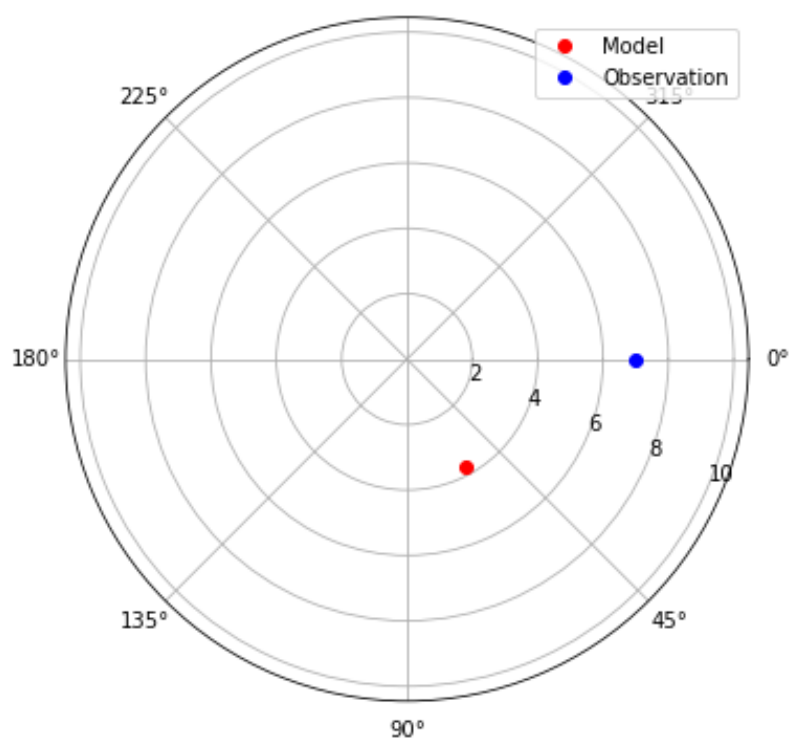
Taylor Diagram - Bushehr Station model (Surface Temperature - CAMS-CSM-01 - SSP.585)
