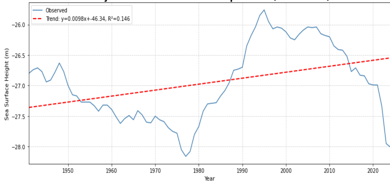
Projected Sea Level in the Caspian Sea (1941-2024)
