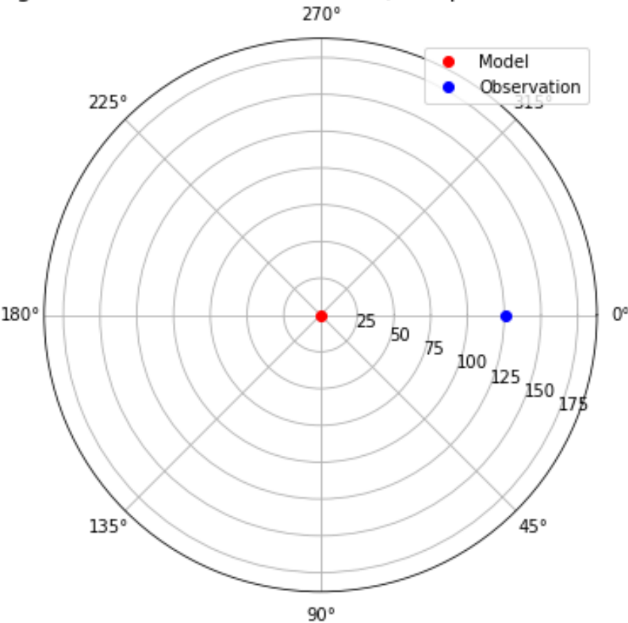
Taylor Diagram - Bushehr Station model (Precipitation-CESM2-SSP.370)
