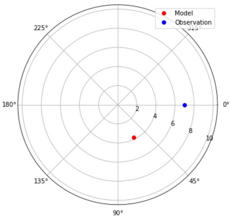
Taylor Diagram - Bushehr Station model (Precipitation-CAMS-CSM-01-SSP.370)
