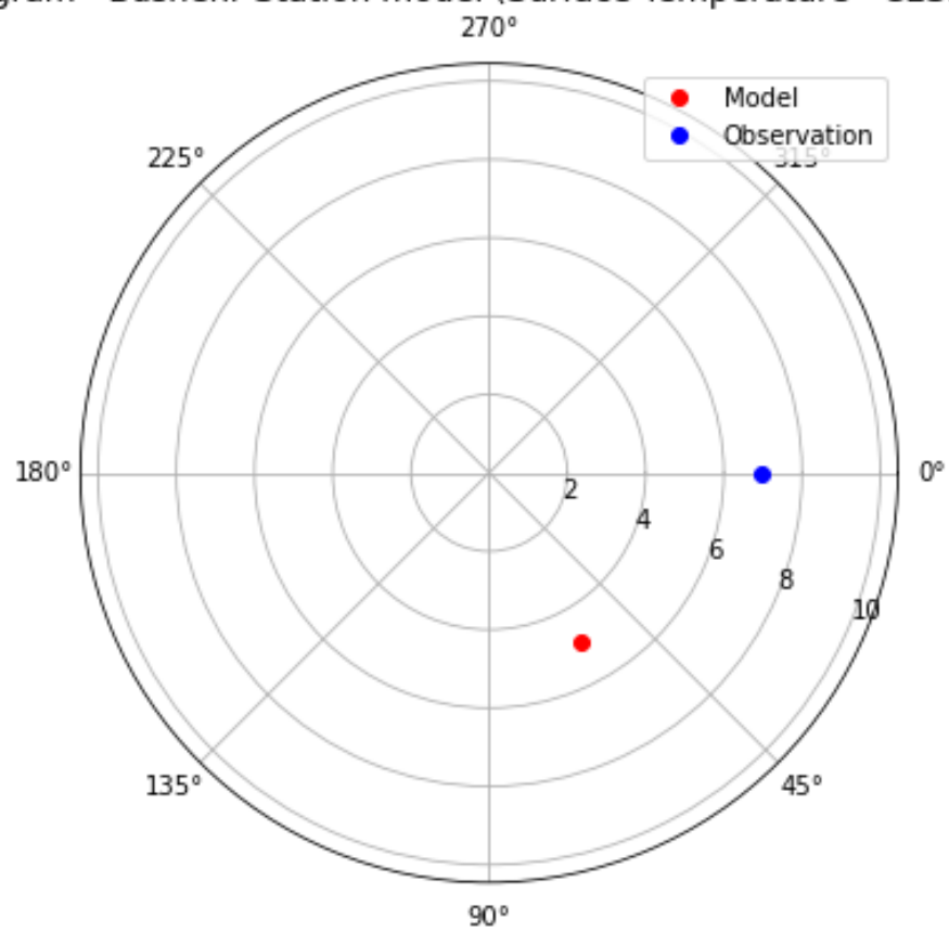
Taylor Diagram - Bushehr Station model (Surface Temperature - CESM2-SSP.585)
