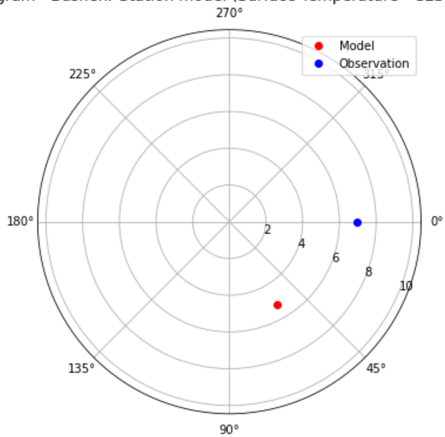
Taylor Diagram - Bushehr Station model (Surface Temperature - CESM2-SSP.370)
