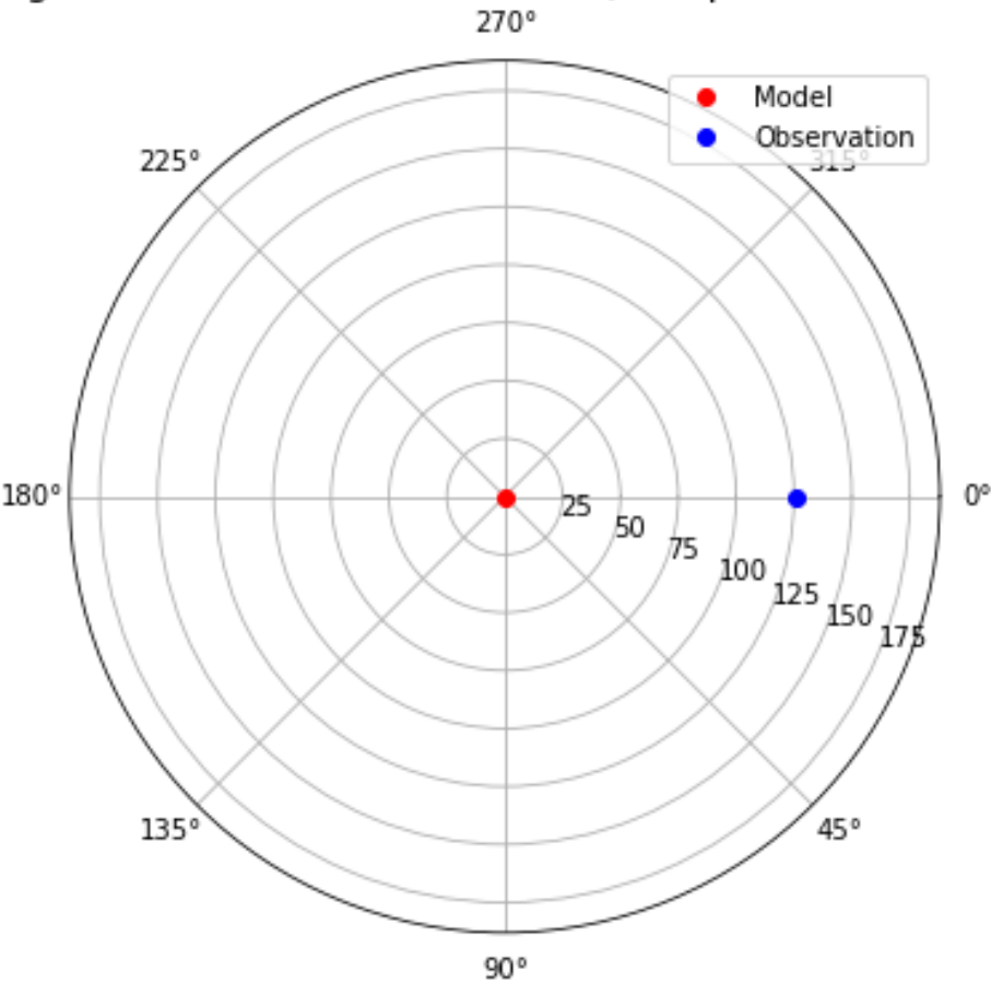
Taylor Diagram - Bushehr Station model (Precipitation-CESM2-SSP.126)
