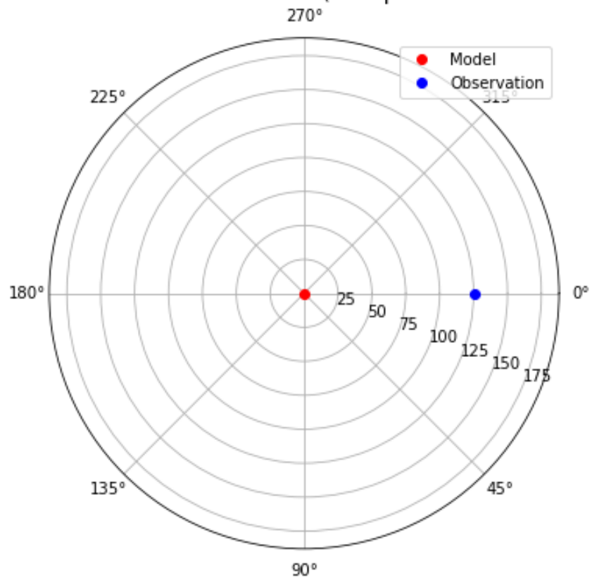
Taylor Diagram - Bushehr Station model (Precipitation-CAMS-CSM1-0-SSP.126)
