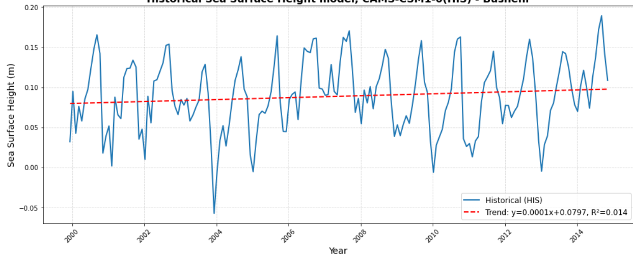
Historical Sea Surface Height model, CAMS-CSM1-0(HIS) - Bushehr
