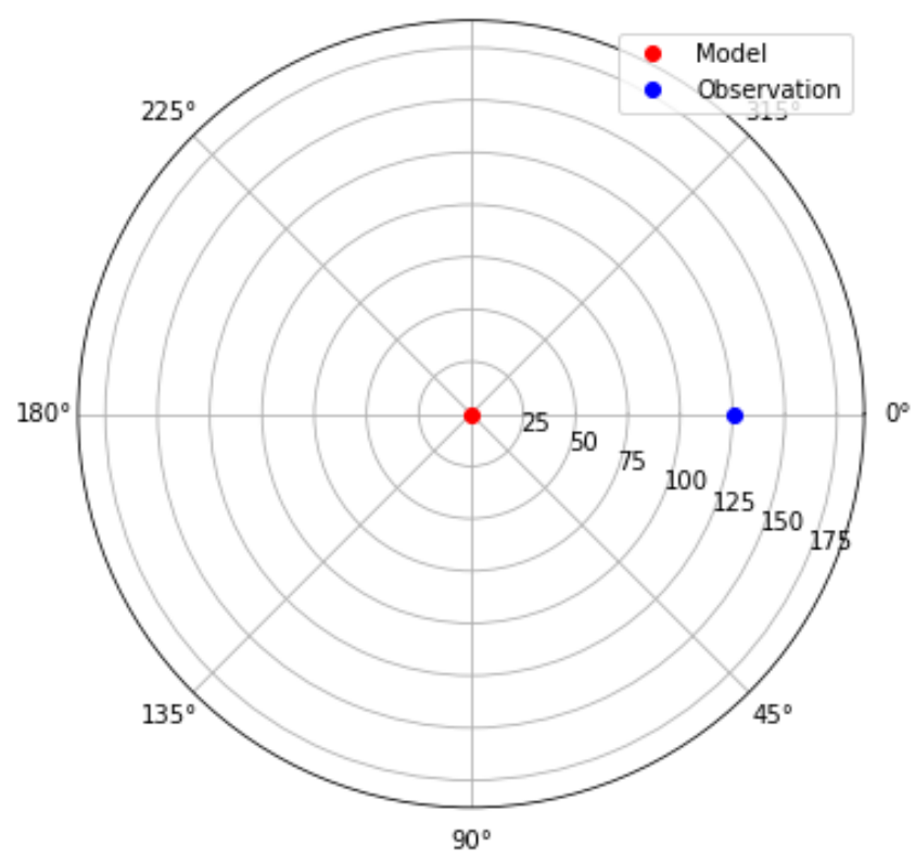
Taylor Diagram - Bushehr Station model (Precipitation-CAMS-CSM-01-SSP.370)
