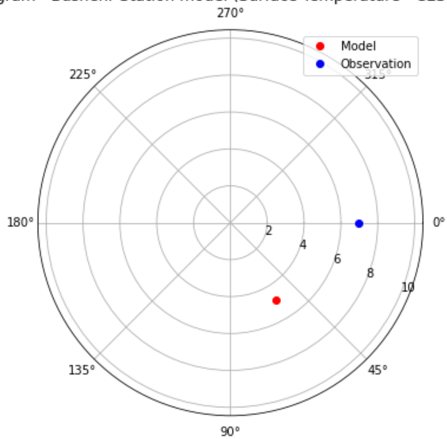
Taylor Diagram - Bushehr Station model (Surface Temperature - CESM2-SSP.126)
